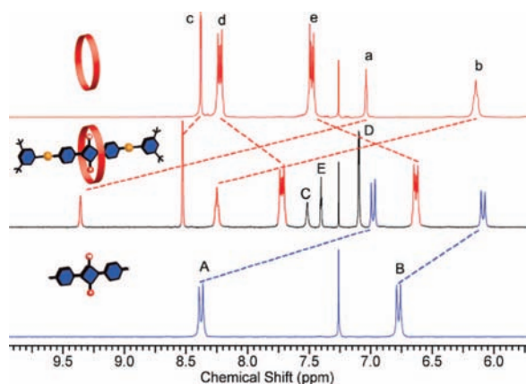
Figure 3. Partial ^1\text{H} NMR spectra of M3 (top), D1 (bottom), and the resulting clicked rotaxane M3>T3 (middle).
