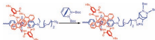
Scheme 3. Capping of Pseudorotaxane M3>D2 To Produce M3>T3
